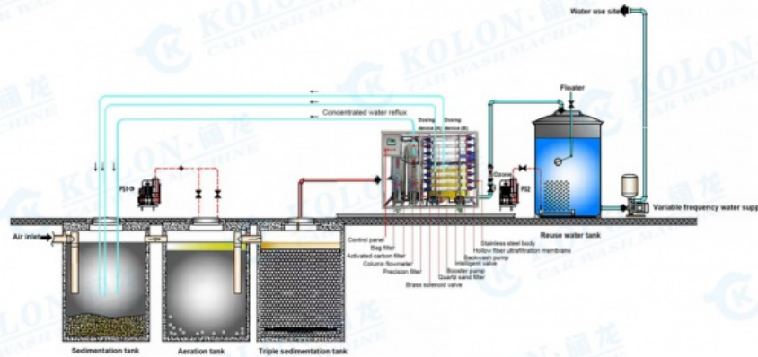
FLOW CHART OF CIRCULATING WATER TREATMENT EQUIPMENT FOR CAR WASHING
